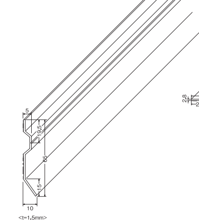
●K-1 ℓ=2000
