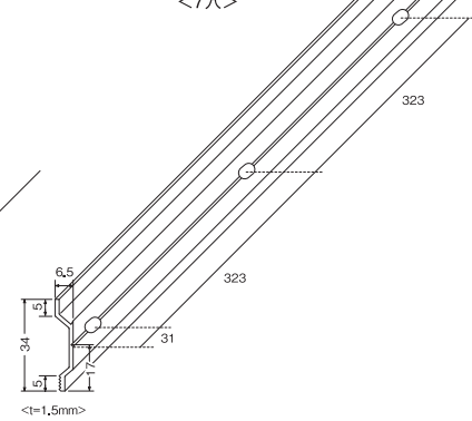
●K-8 ℓ=2000 <7穴>
